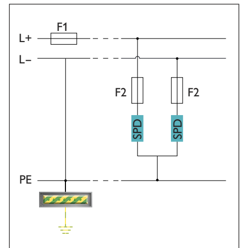
Fig. 64: 2+0 circuit for grounded TN systems that are far away from the grounding point
