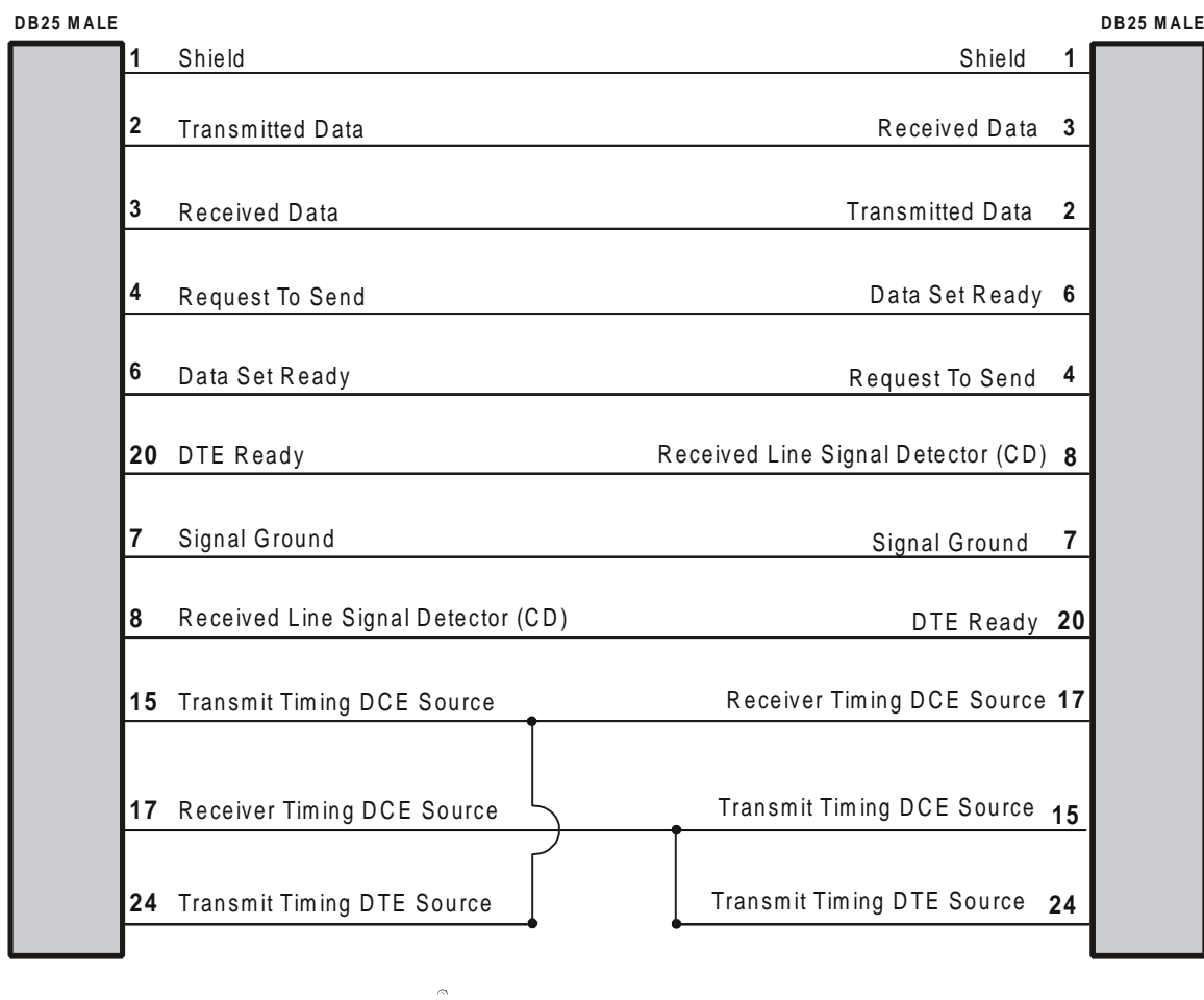
Figure 3 - 11 RS232 Null-Modem Cable
