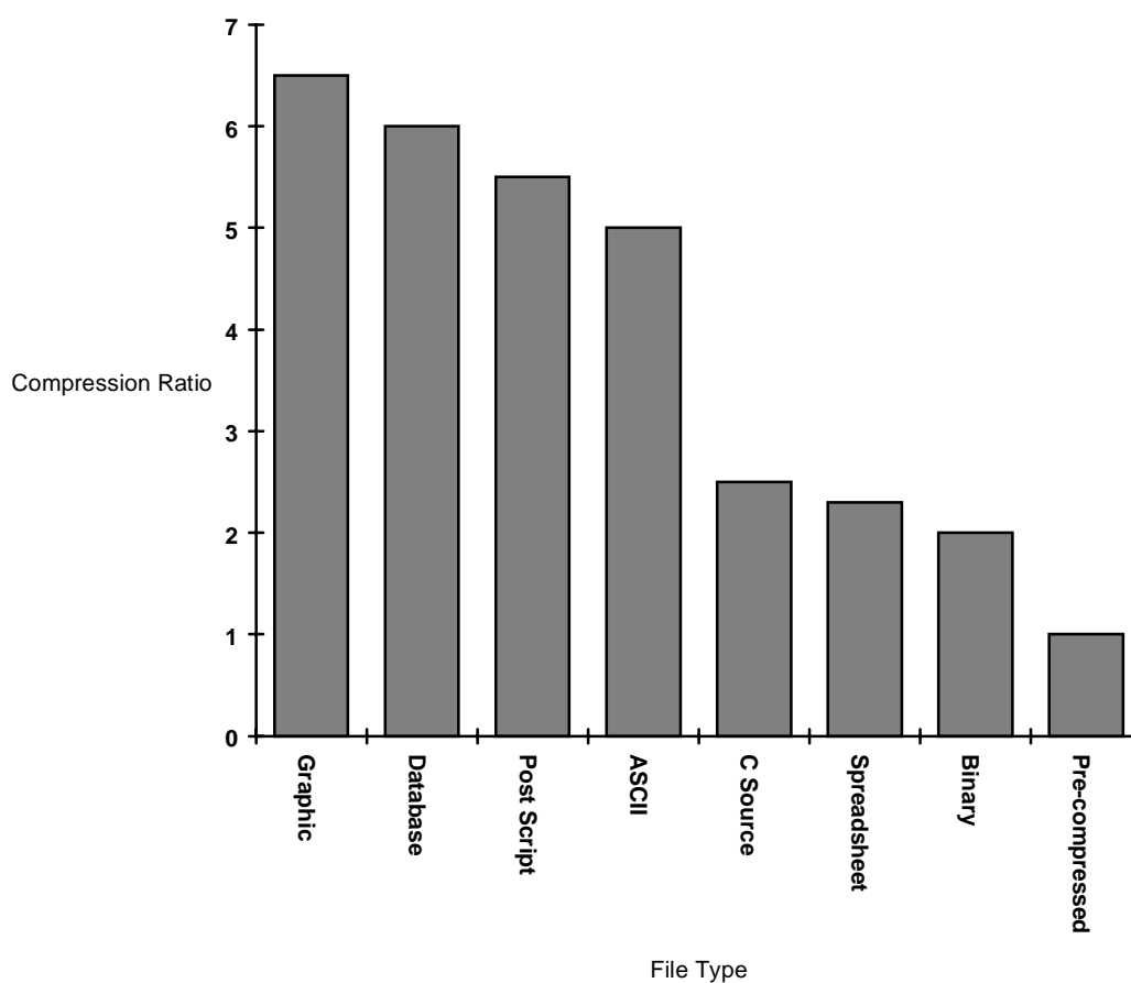
Figure 1 - 5 Typical Compression Ratios by File Type
