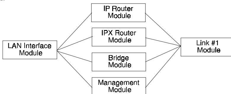
Figure 1 - 1 P850 Ethernet Bridge/Router Block Diagram
