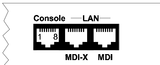
Figure 2-1 Rear View of the Console Connector
