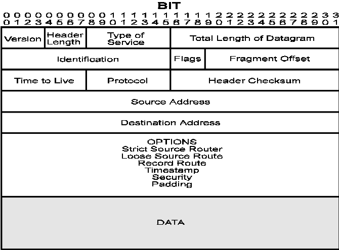
Figure 1 - 2 IP Header
