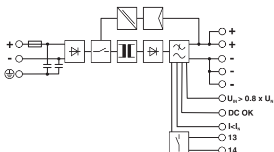
Figure 1 Basic circuit diagram
