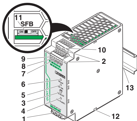
Figure 2 Function elements
